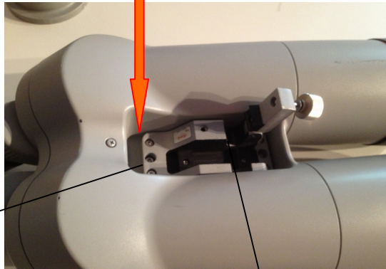
Holder for center mount (included in center-mount package)
